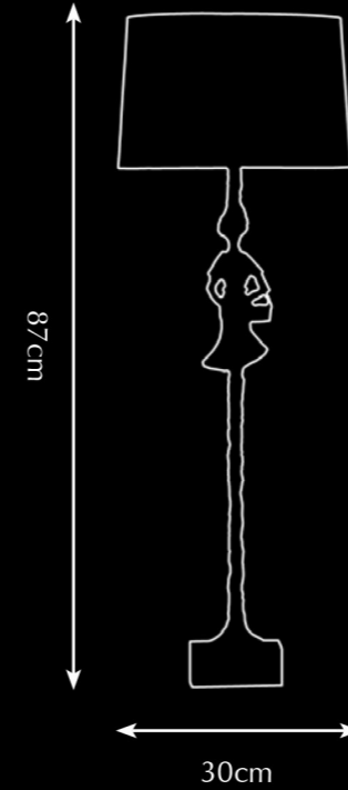
Itemnr: PA 850 Model: Melting Paris Sunday afternoon woman Material: Casted brass Shade: 8261 Burnished Gold Velvet Sockets: 2x E14 max. 40 Watt Finishes: -Dutch Silver -Canadian Gold -Smoked Brass
