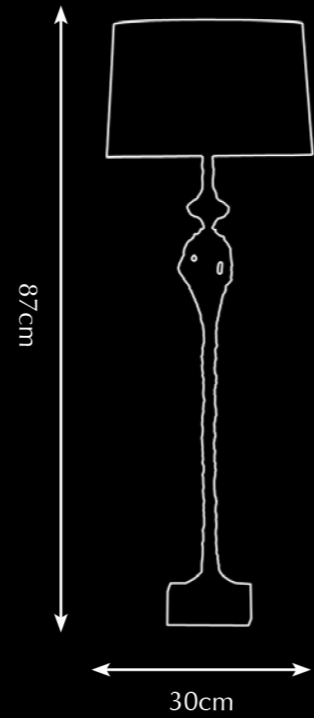
Itemnr: PA 851 Model: Melting Paris Sunday afternoon man Material: Casted brass Shade: 8261 Burnished Gold Velvet Sockets: 2x E14 max. 40 Watt Finishes: -Dutch Silver -Canadian Gold -Smoked Brass
